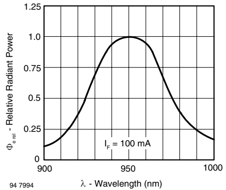
94 7994 Fig. 9 - Relative Radiant Power vs. Wavelength
