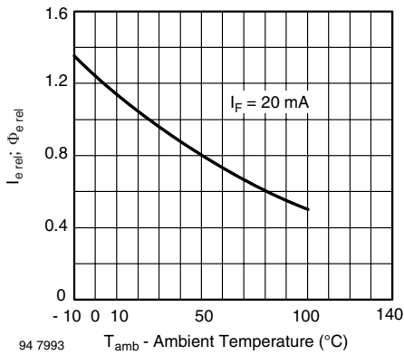
94 7993 Fig. 8 - Relative Radiant Intensity/Power vs. Ambient Temperature
