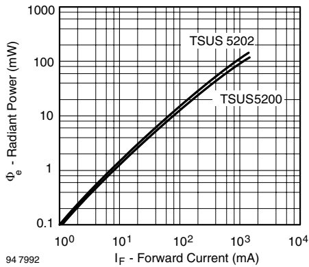
94 7992 Fig. 7 - Radiant Power vs. Forward Current
