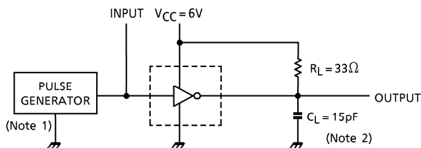
7. t_{ON} , t_{OFF}
