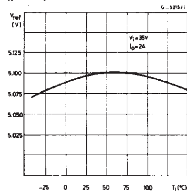
Figure 9. Reference voltage versus junction temperature (pin 2)
