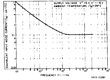
Fig.5— I_N vs. Frequency for CA6741T.
