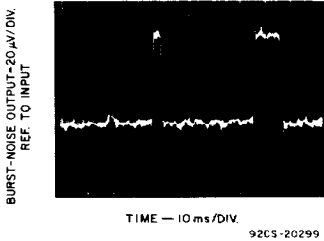
a. Typ. device with high-burst-noise characteristic.
