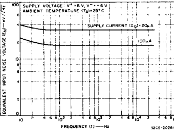
Fig.4— E_N vs. Frequency for CA6078AT.
