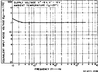
Fig.6— E_N vs. Frequency for CA6741T.
