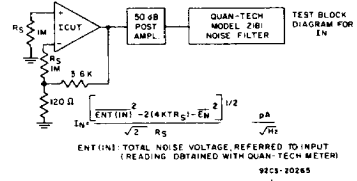
Fig.8—Test block diagram for I_N .
