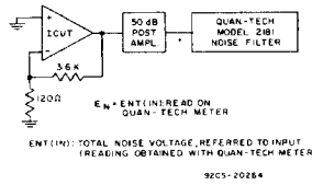
Fig.7—Test block diagram for E_N .
