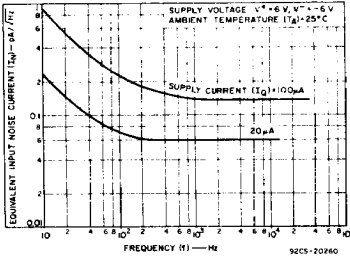
Fig.3— I_N vs. Frequency for CA6078AT.
