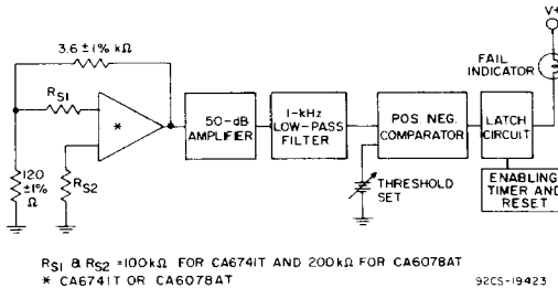
Fig.2—Block diagram of burst-noise "popcorn" test equipment.
