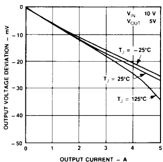
Load Regulation
