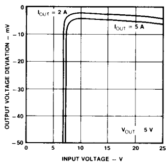
Line Regulation
