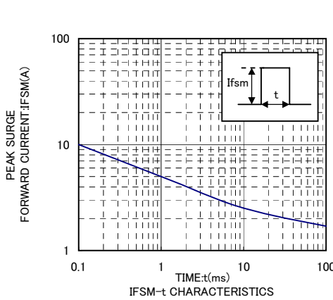
IFSM-t CHARACTERISTICS
