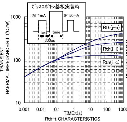
Rth-t CHARACTERISTICS
